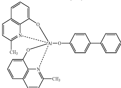
BAIq
